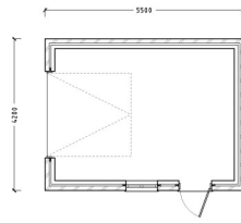
Garage Layout. 1:50.
